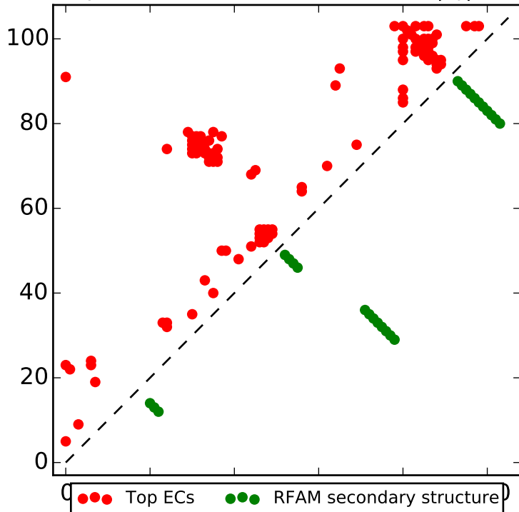
Top L contacts for RF01867 with |i-j| > 4
