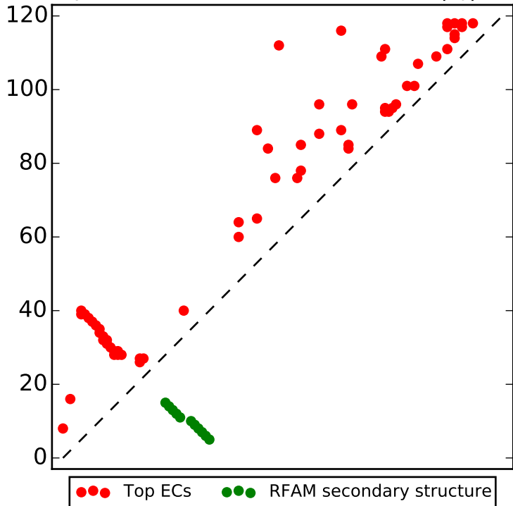
Top L/2 contacts for RF01942 with |i-j| > 4
