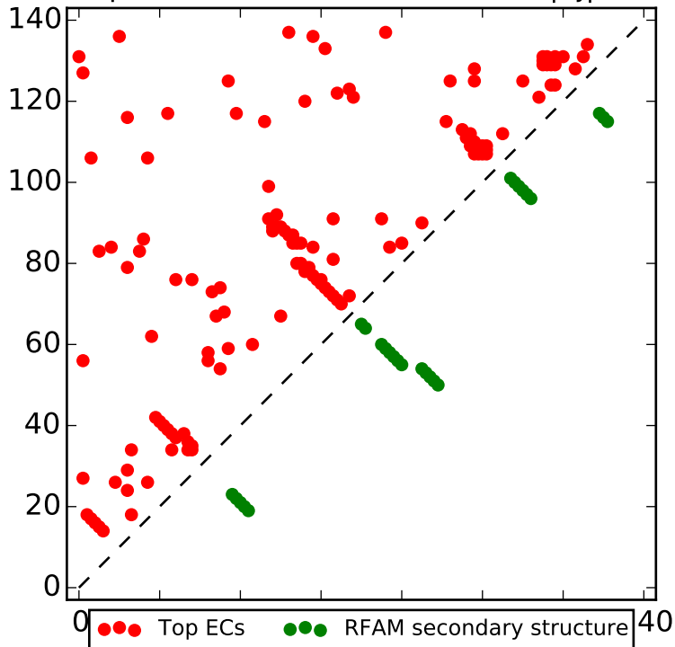
Top L contacts for RF02003 with |i-j| > 4
