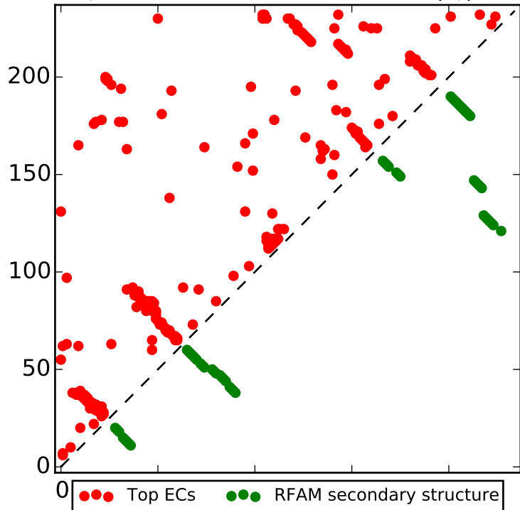
Top L contacts for RF02005 with |i-j| > 4
