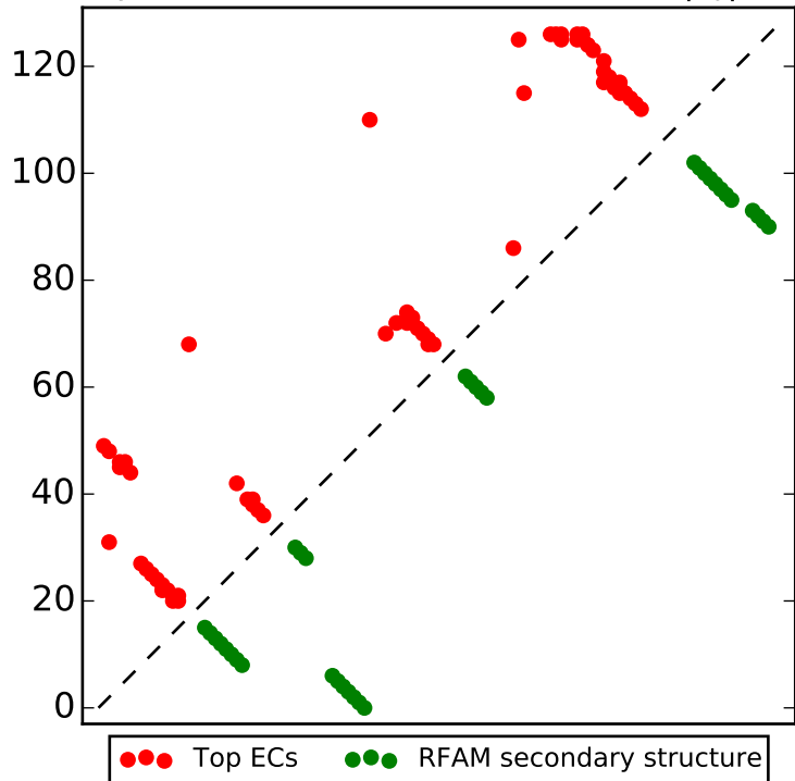
Top L/2 contacts for RF02033 with |i-j| > 4
