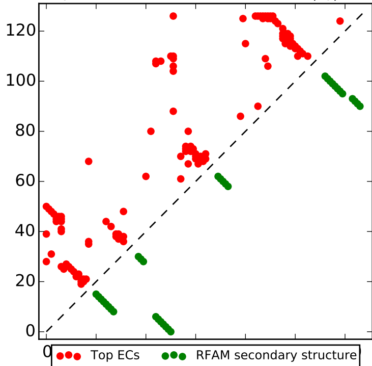
Top L contacts for RF02033 with |i-j| > 4
