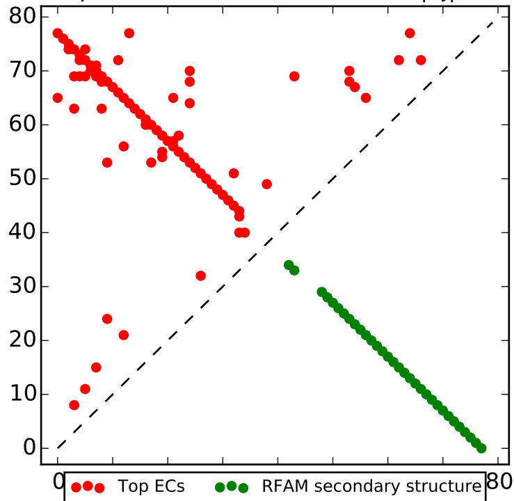
Top L contacts for RF02096 with |i-j| > 4
