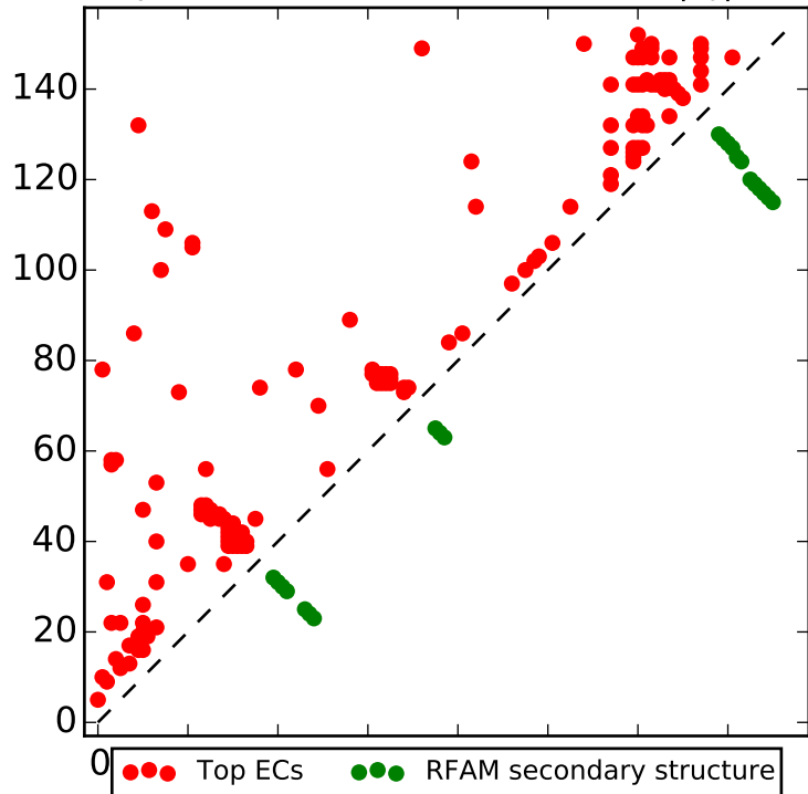
Top L contacts for RF02194 with |i-j| > 4
