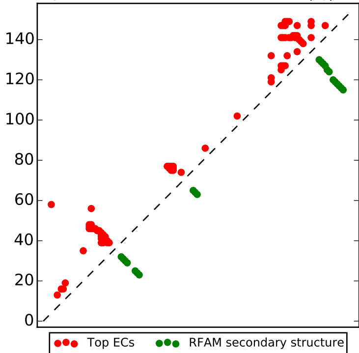
Top L/2 contacts for RF02194 with |i-j| > 4
