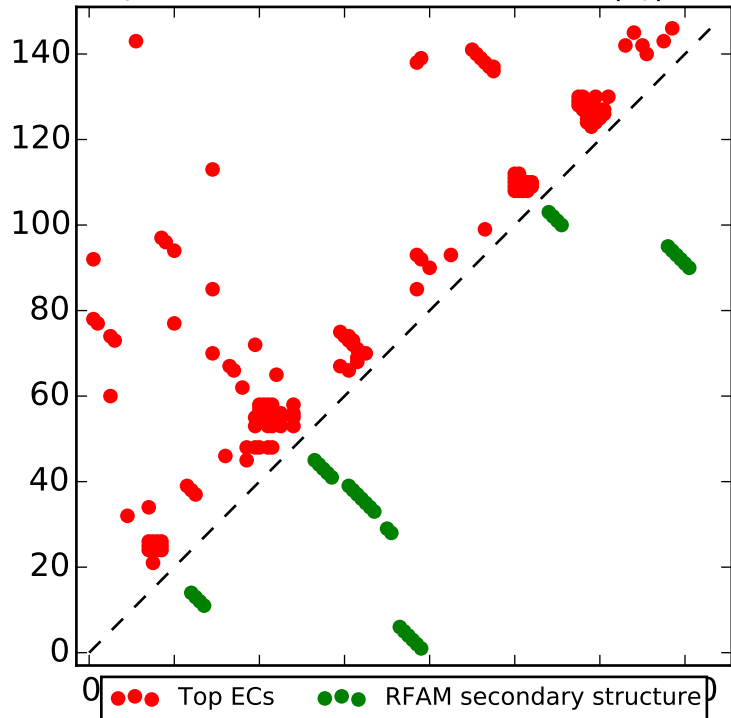
Top L contacts for RF02223 with |i-j| > 4
