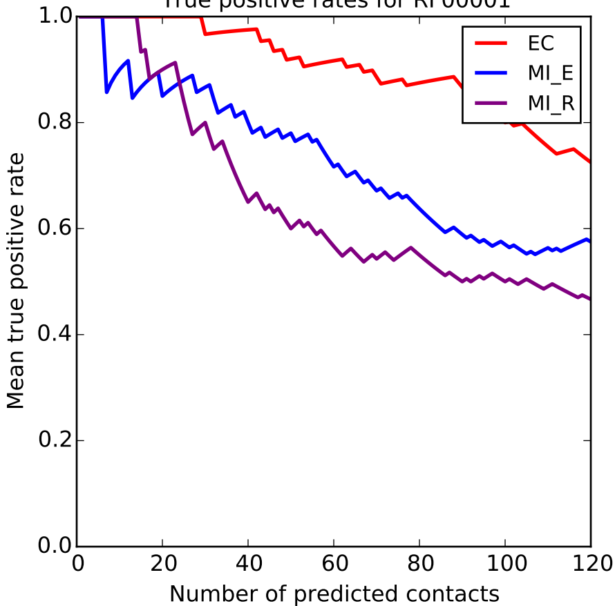
True positive rates for RF00001
