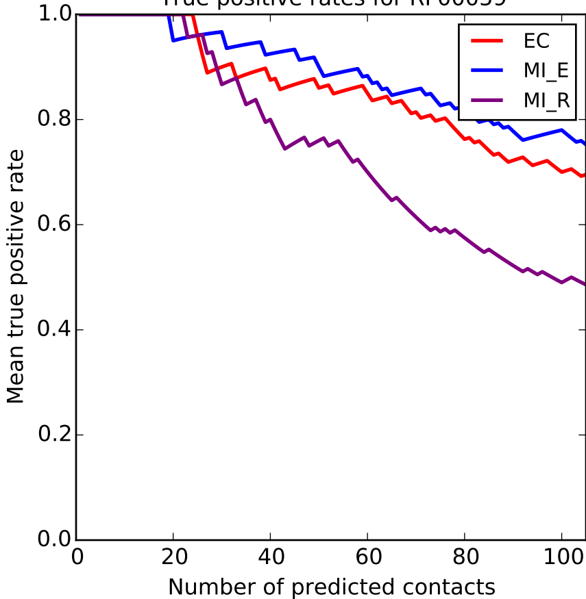
True positive rates for RF00059
