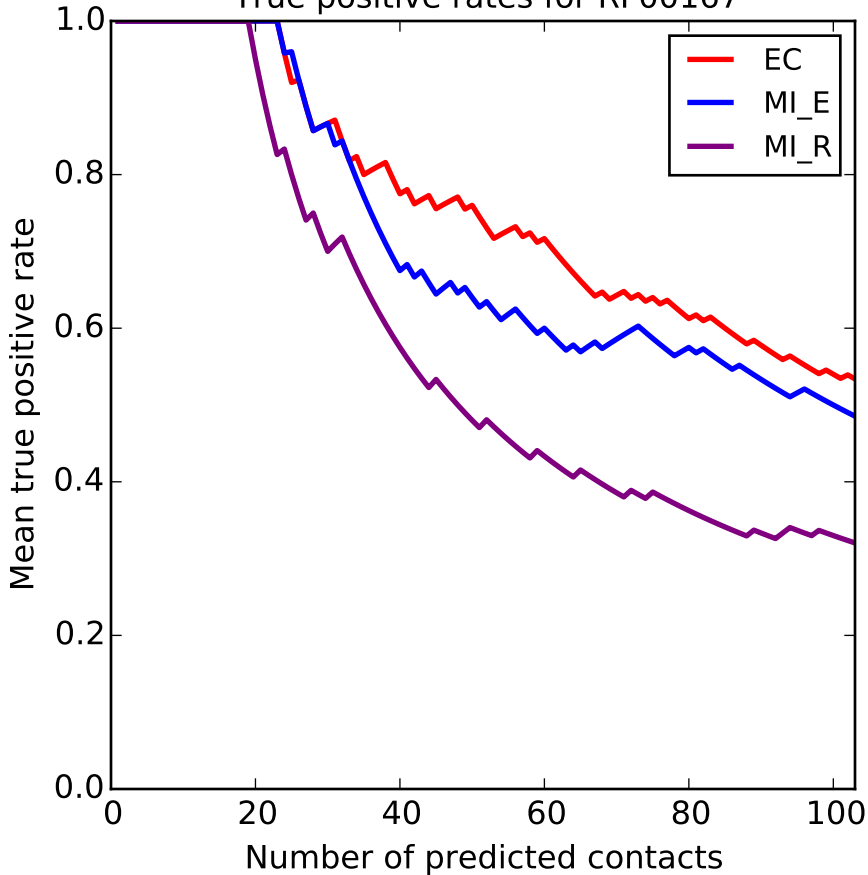
True positive rates for RF00167
