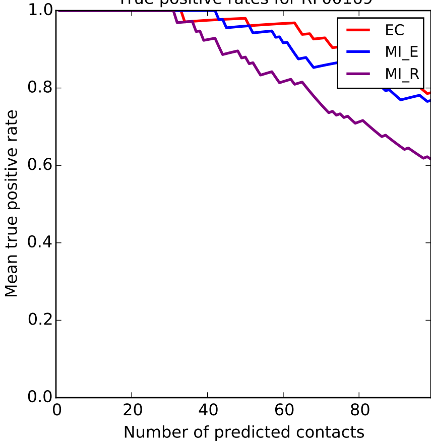
True positive rates for RF00169
