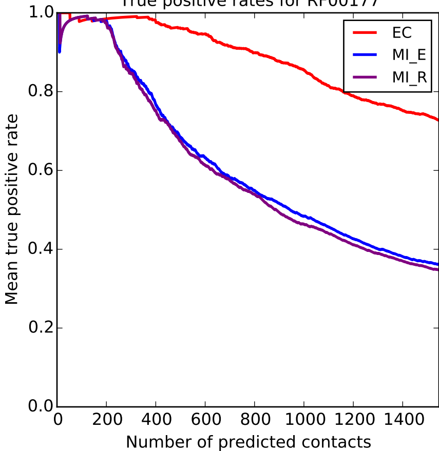
True positive rates for RF00177
