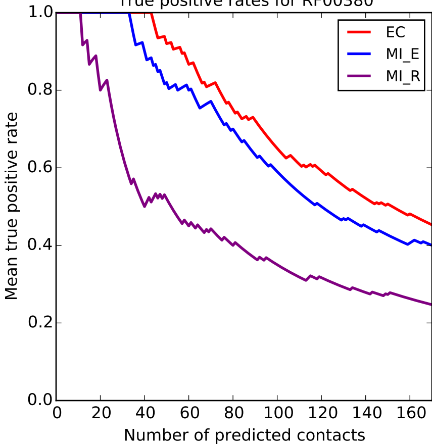
True positive rates for RF00380
