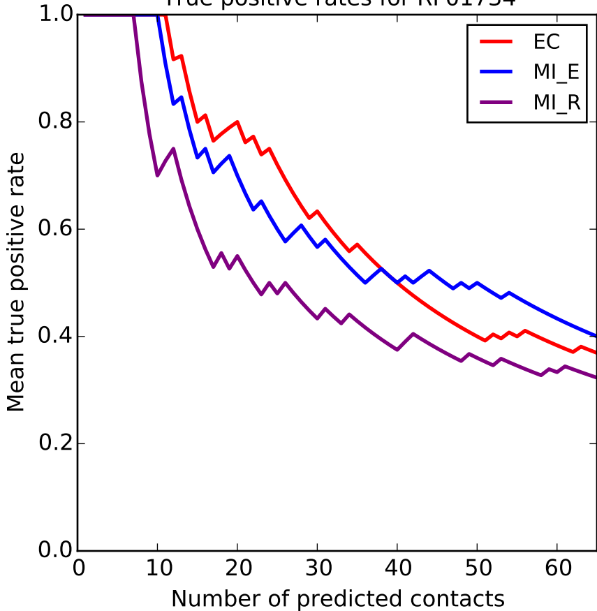
True positive rates for RF01734
