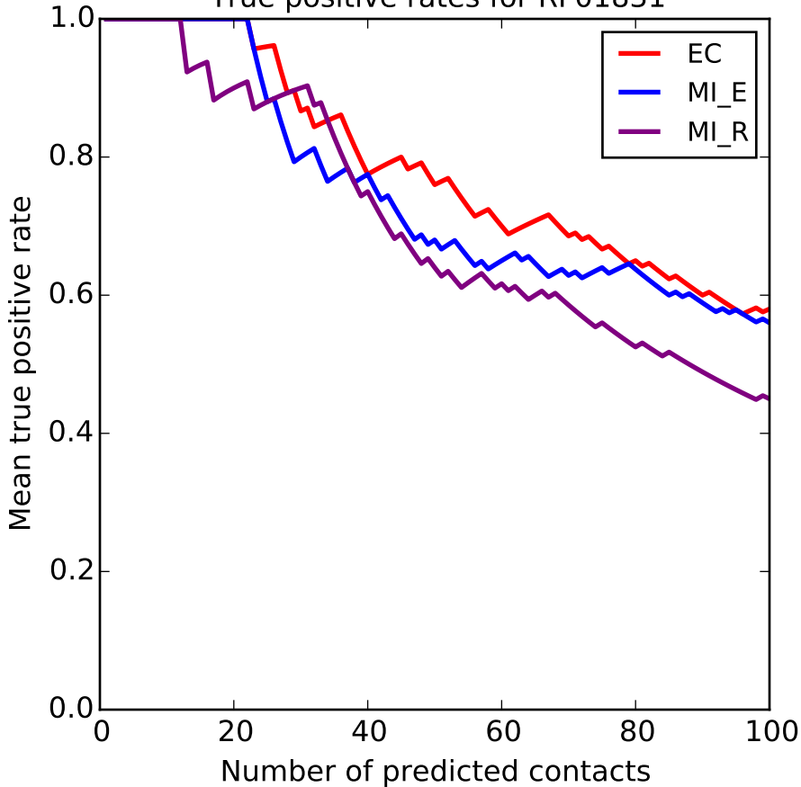
True positive rates for RF01831
