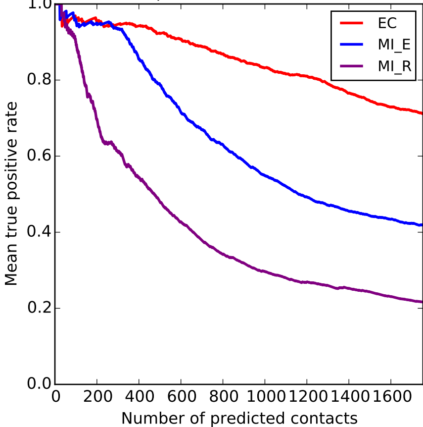
True positive rates for RF01960
