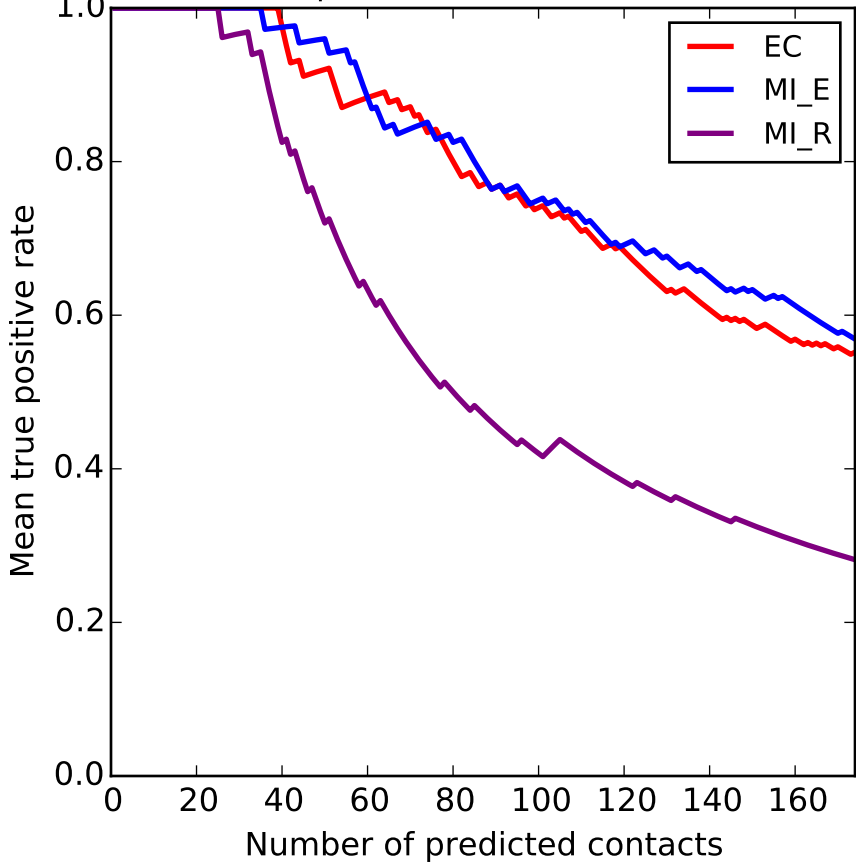
True positive rates for RF02001
