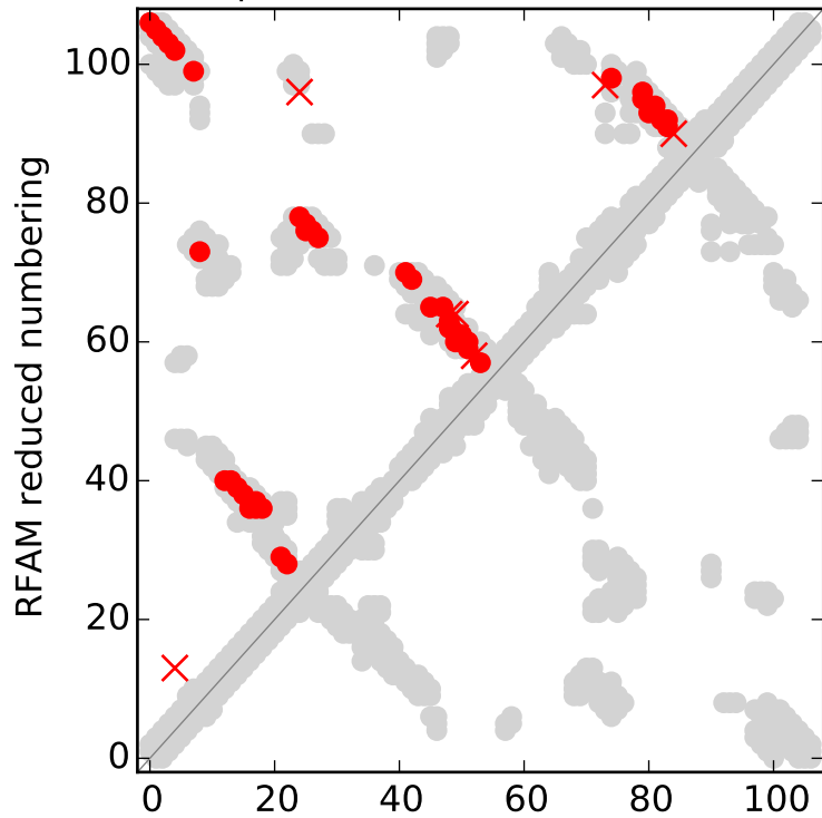
Top L EC contacts for RF00162
