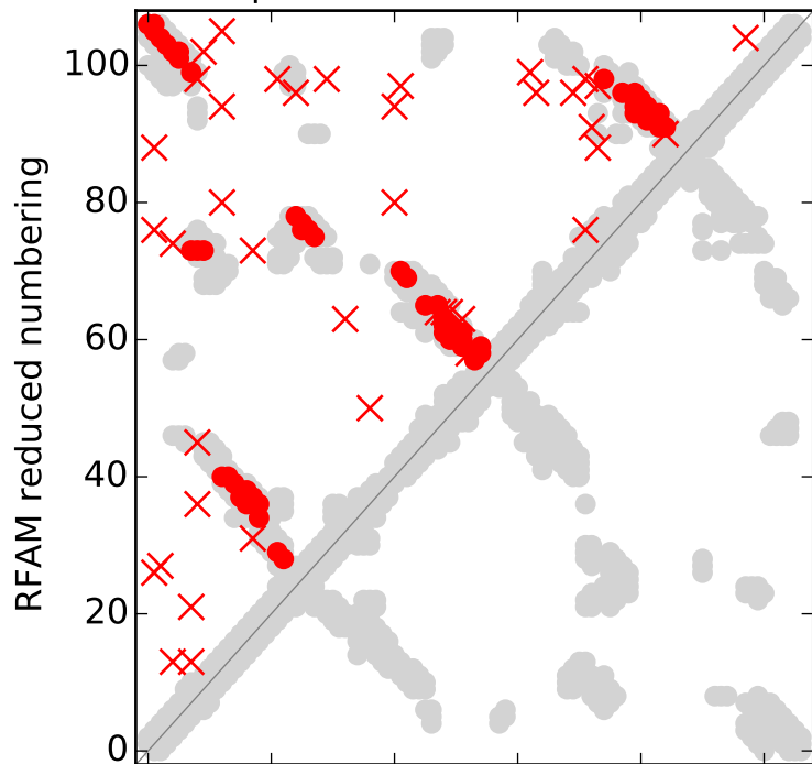
Top L EC contacts for RF00162
