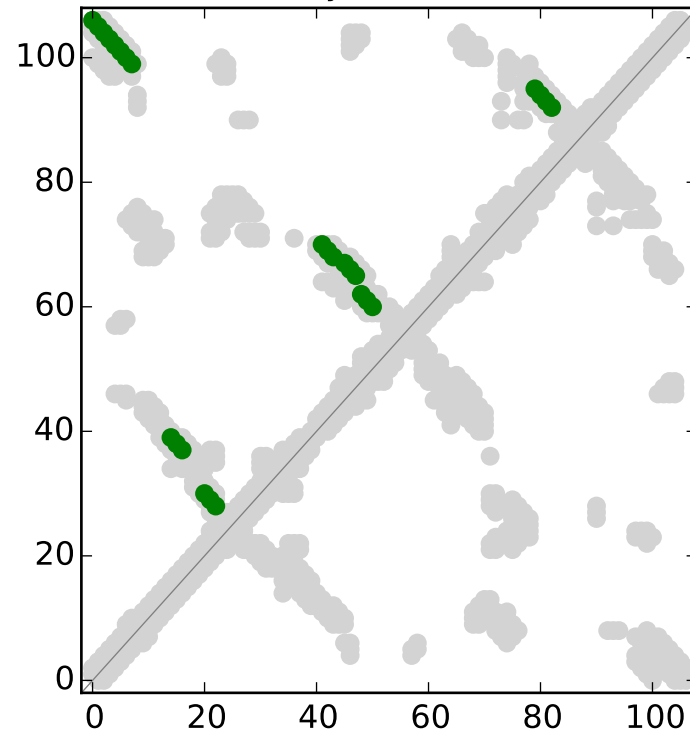
RFAM secondary structure for RF00162
