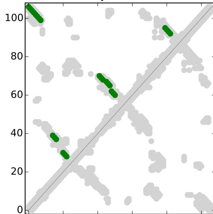
RFAM secondary structure for RF00162
