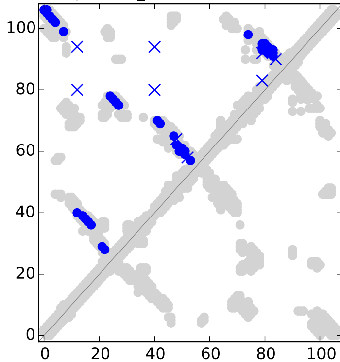
Top L MI_E contacts for RF00162
