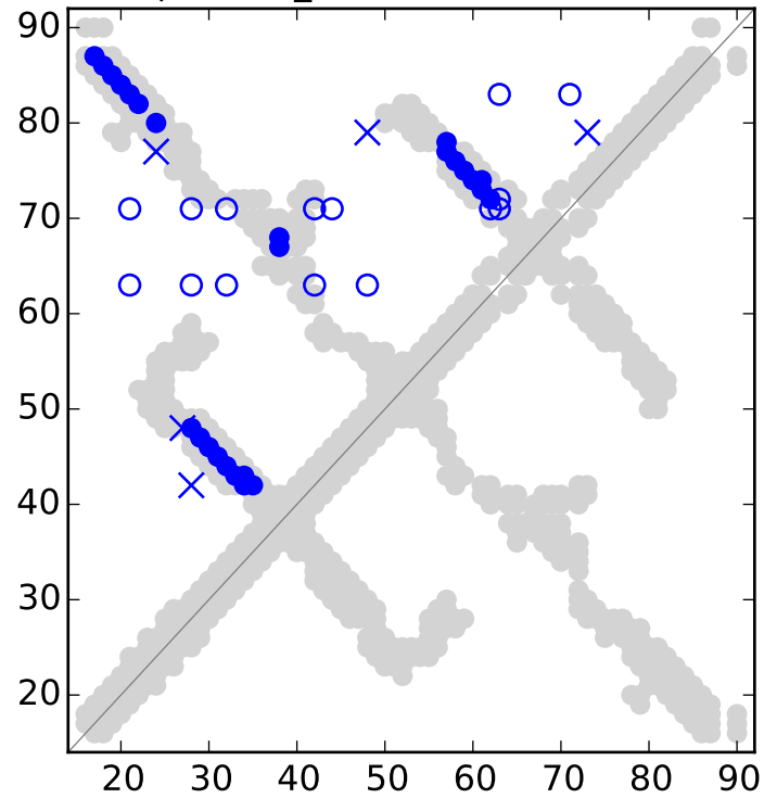
Top L/2 MI_E contacts for RF00167
