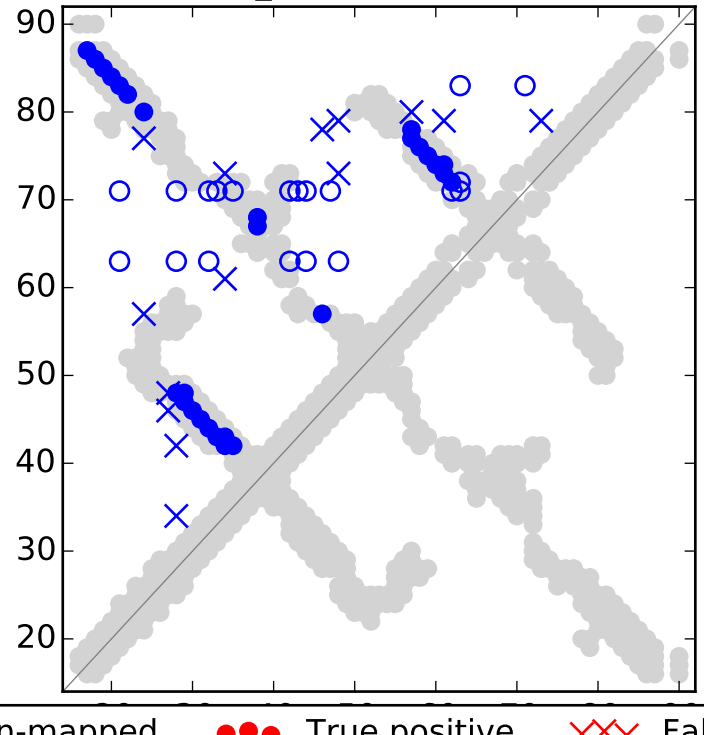
Top L MI_E contacts for RF00167
