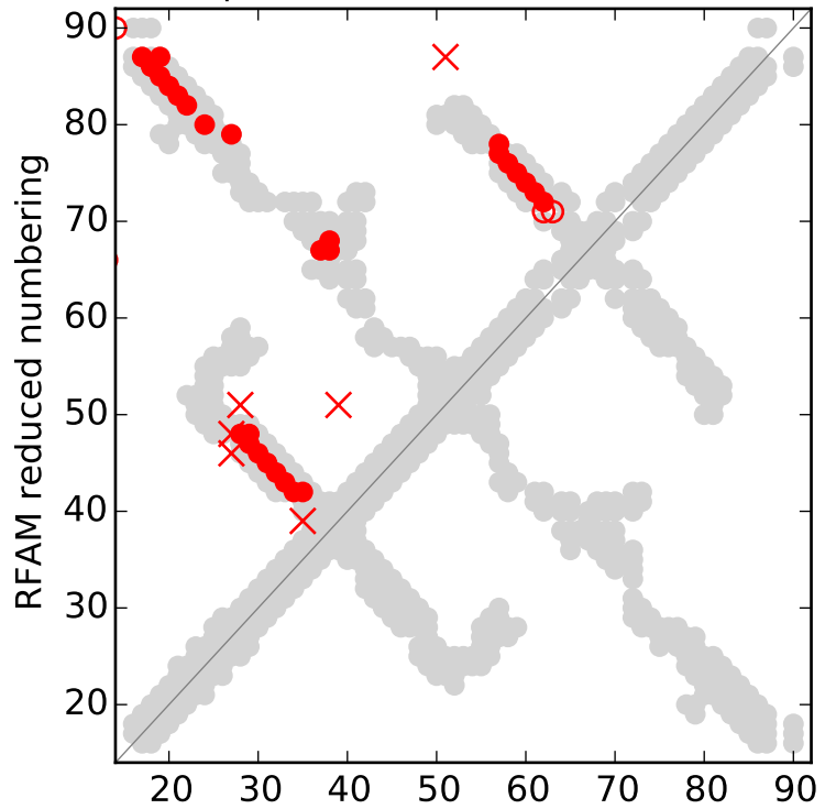
Top L/2 EC contacts for RF00167
