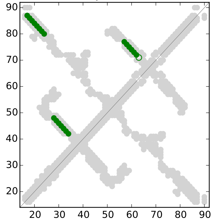
RFAM secondary structure for RF00167
