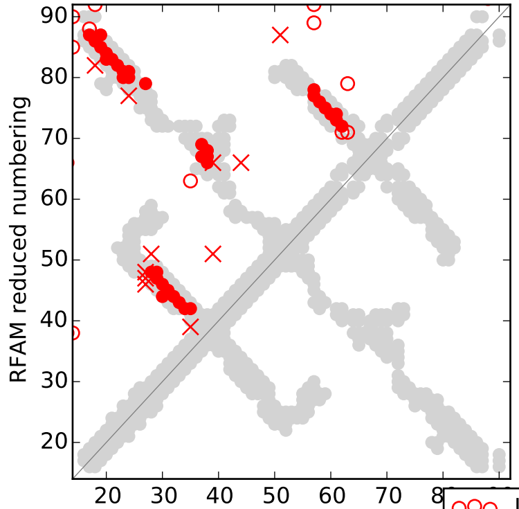
Top L EC contacts for RF00167
