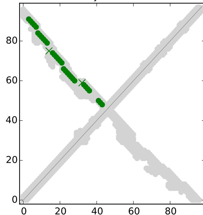
RFAM secondary structure for RF00169
