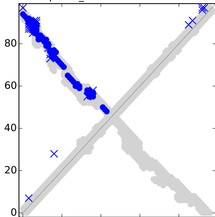
Top L MI_E contacts for RF00169
