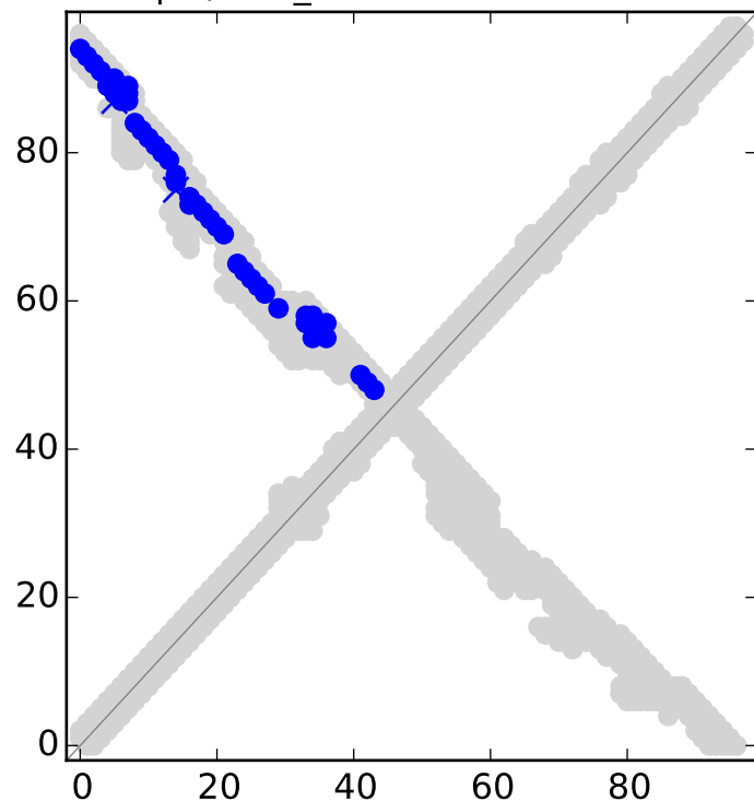
Top L MI_E contacts for RF00169
