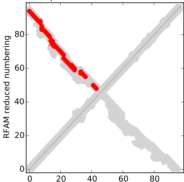
Top L EC contacts for RF00169
