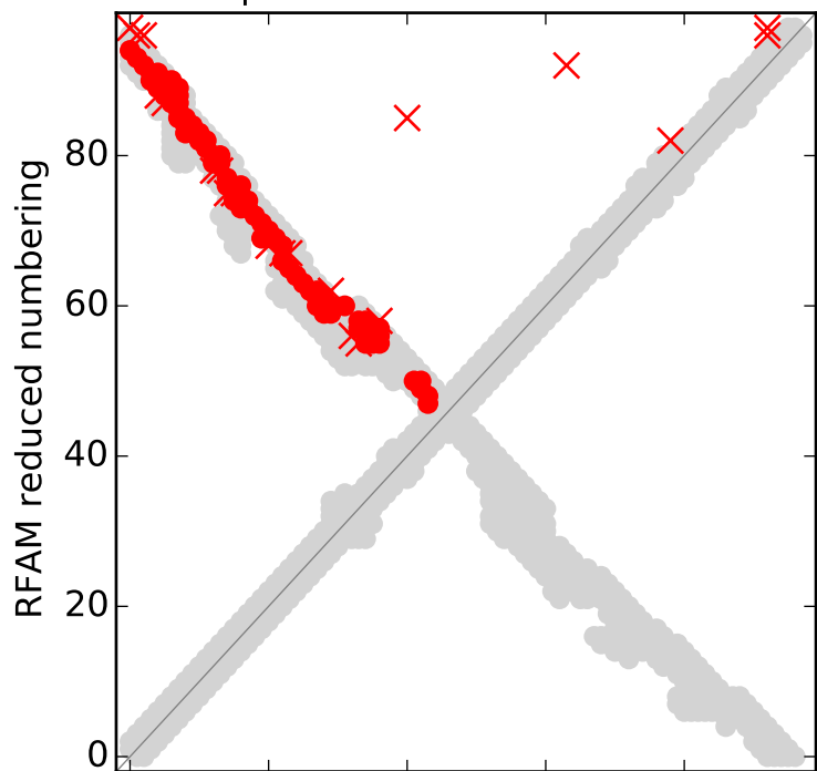
Top L EC contacts for RF00169
