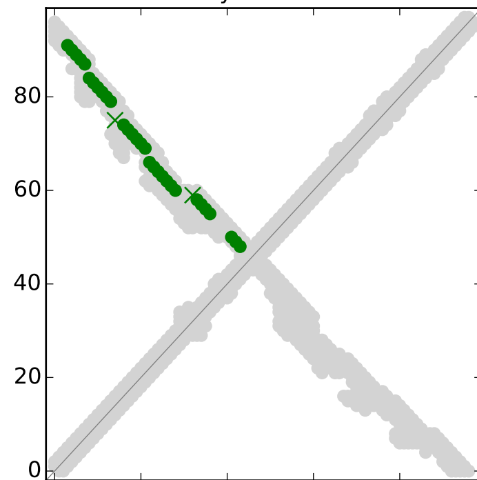
RFAM secondary structure for RF00169
