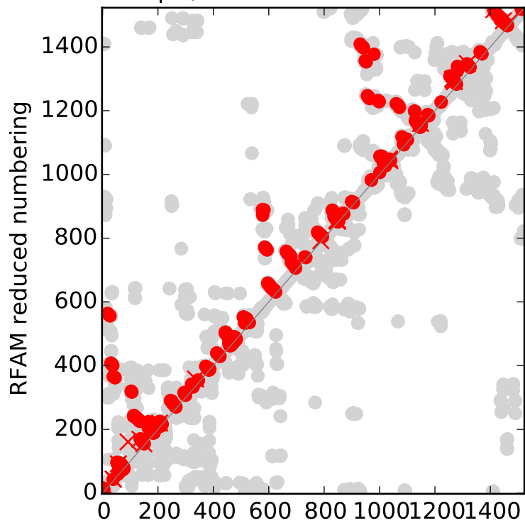
Top L EC contacts for RF00177
