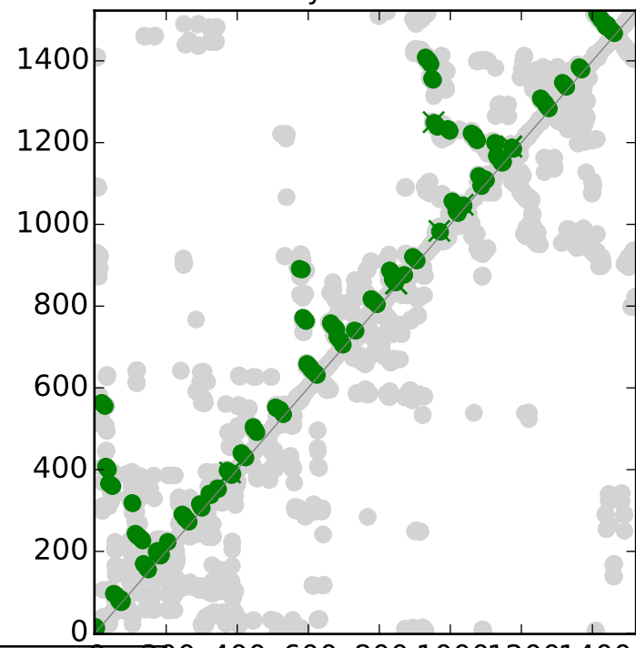
RFAM secondary structure for RF00177
