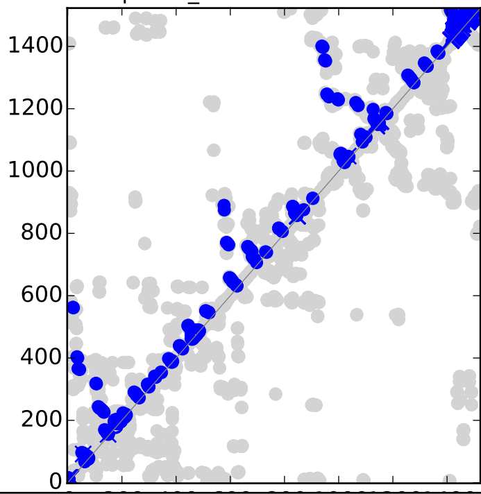
Top L MI_E contacts for RF00177
