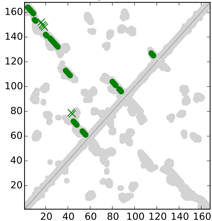
RFAM secondary structure for RF00380
