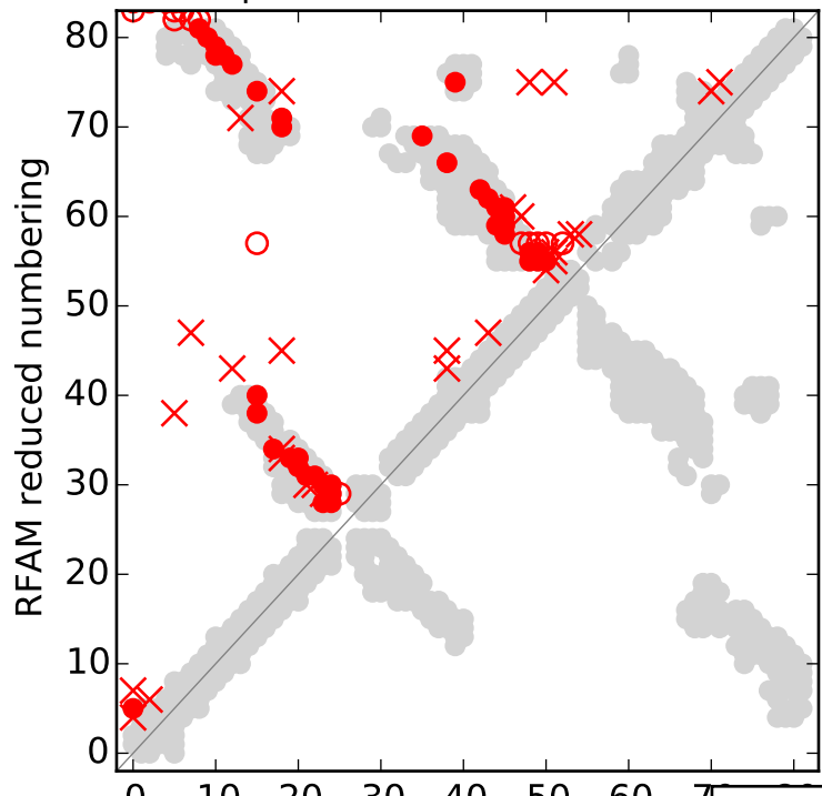
Top L EC contacts for RF00504
