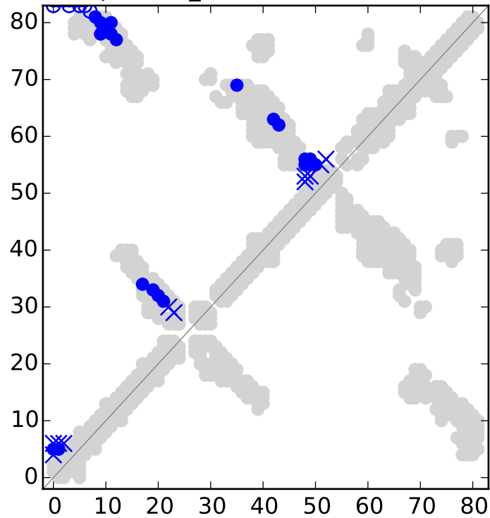
Top L MI_E contacts for RF00504
