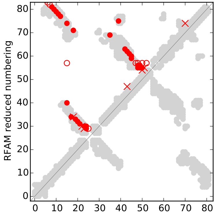
Top L EC contacts for RF00504
