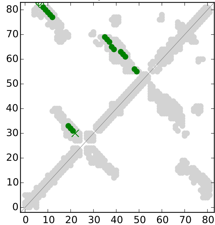
RFAM secondary structure for RF00504
