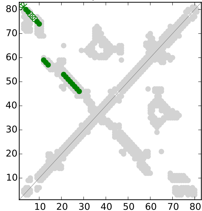
RFAM secondary structure for RF01786
