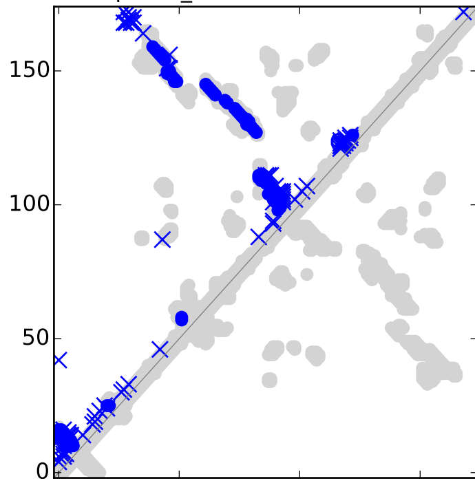
Top L MI_E contacts for RF02001
