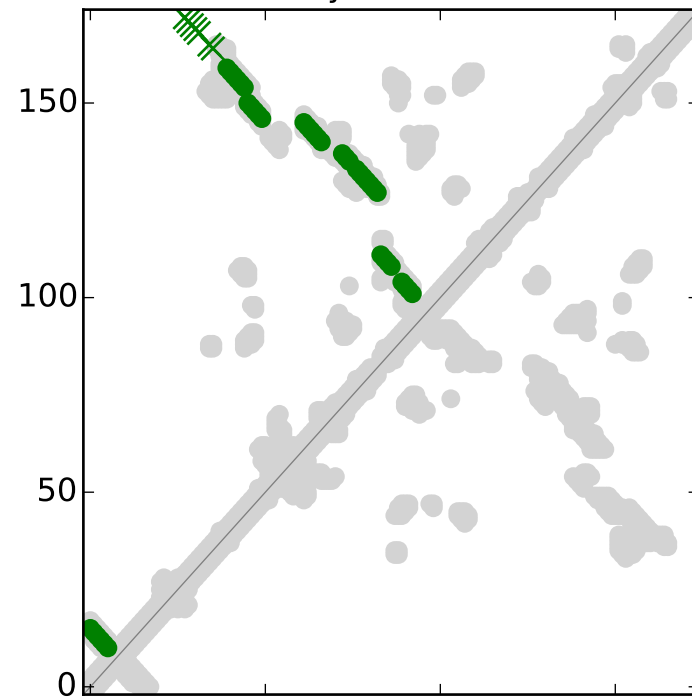
RFAM secondary structure for RF02001
