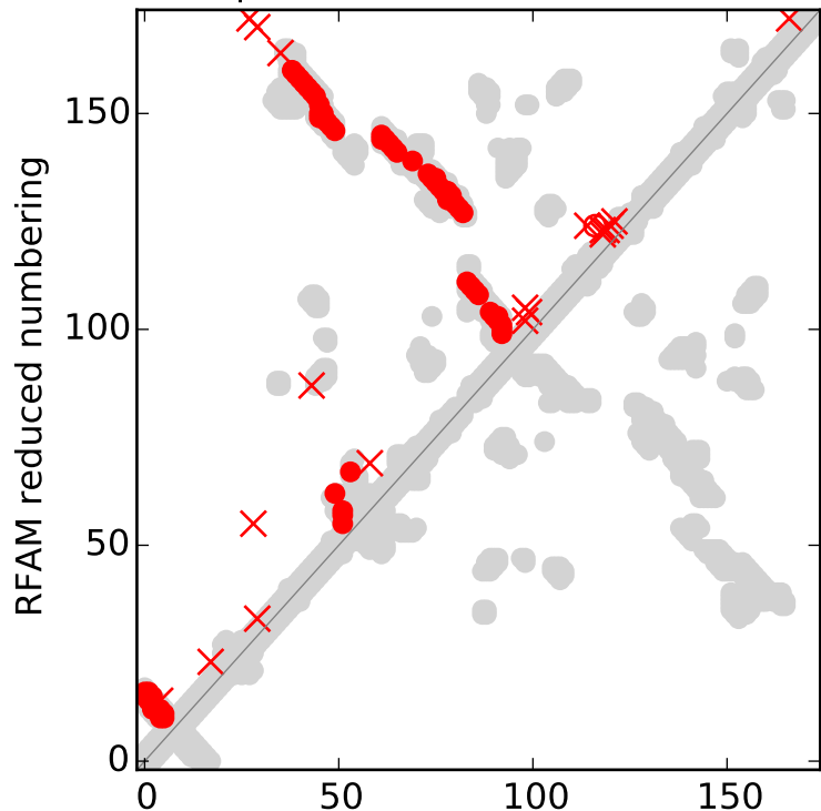
Top L/2 EC contacts for RF02001
